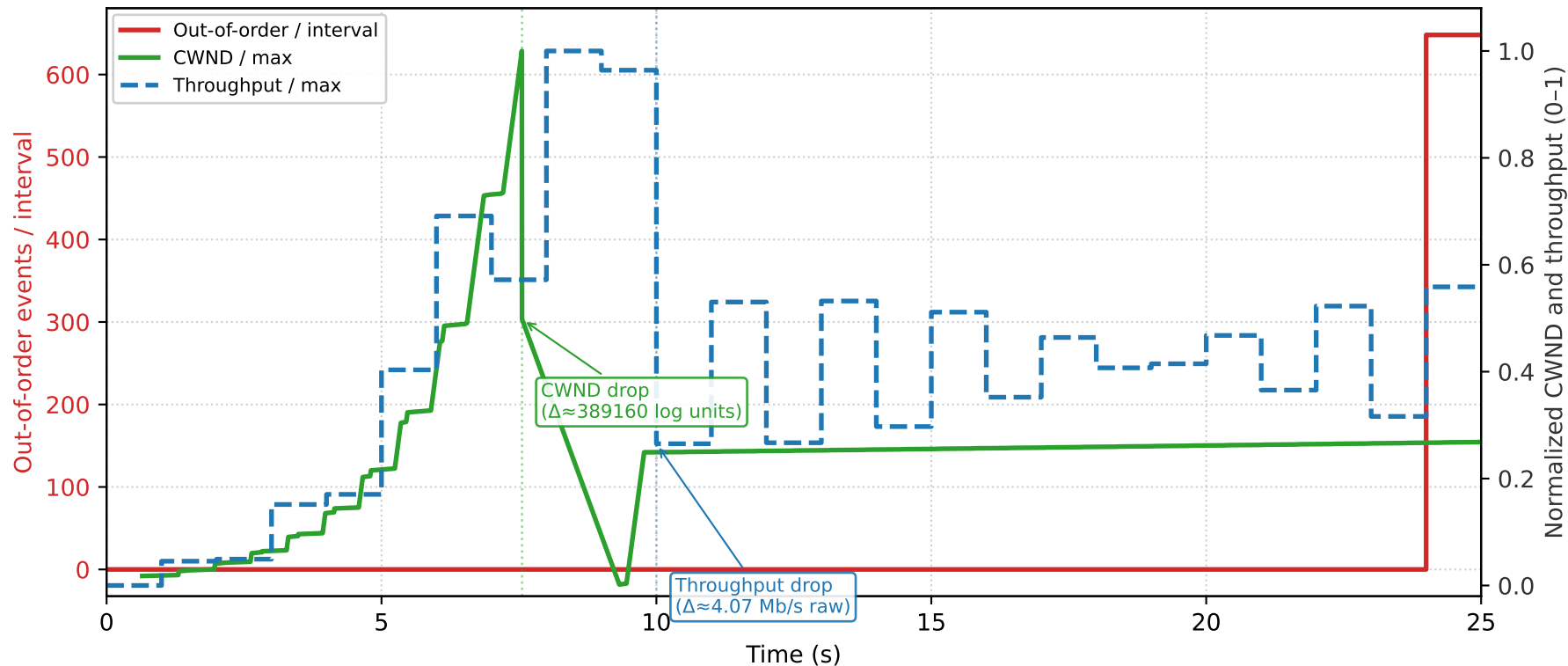
Figure G4 — Out-of-order vs normalized CWND & throughput (Multilayer) — 25 s sim, 1000 ms state updates Case: Tokyo to Buenos-Aires
